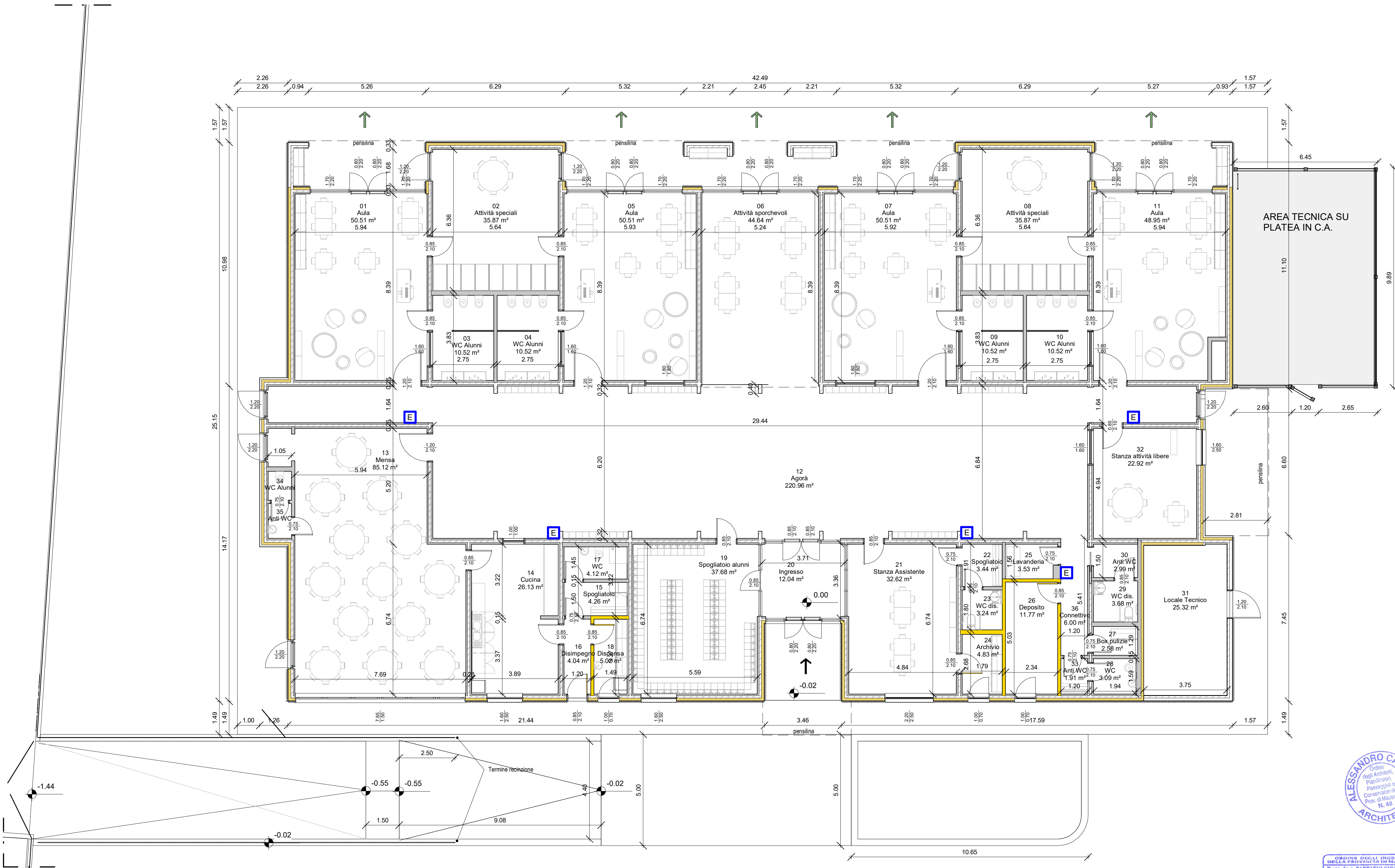
1 Piano Terra 1:100
